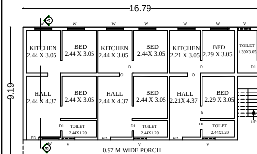
EXG GROUND FLOOR
