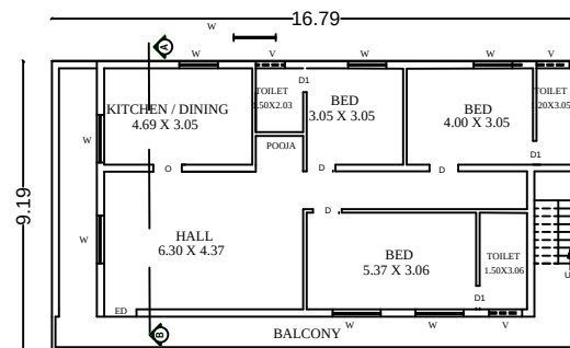
PRO. ADD SECOND FLOOR
