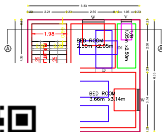
FLOOR PLAN
