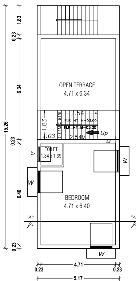
PRO. FIRST FLOOR PLAN
