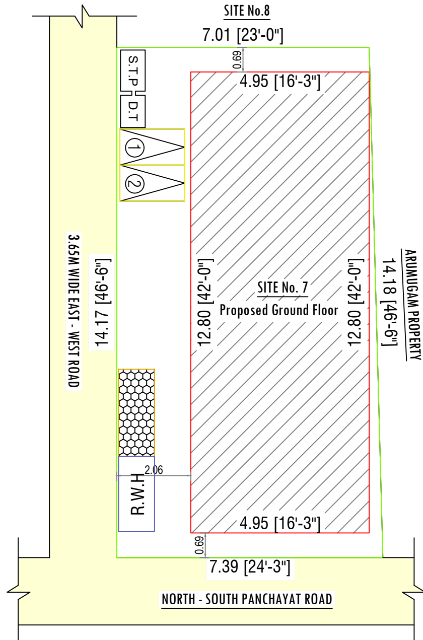
SITE PLAN
