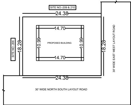
SITE PLAN
