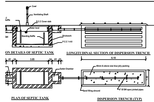
DETAILS OF SEPTIC TANK - 250 GALLONS & DISPERSION TRENCH
