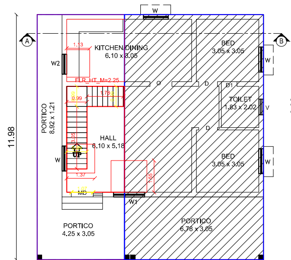
EXISTING & PRO.ADDL.GROUND FLOOR PLAN
