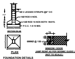
FOUNDATION DETAILS
