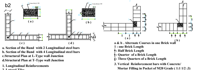
Figure - 2 : Typical Details of Providing Vertical Steel Bars in Brick Masonry.
