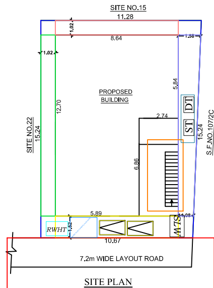
SITE PLAN
