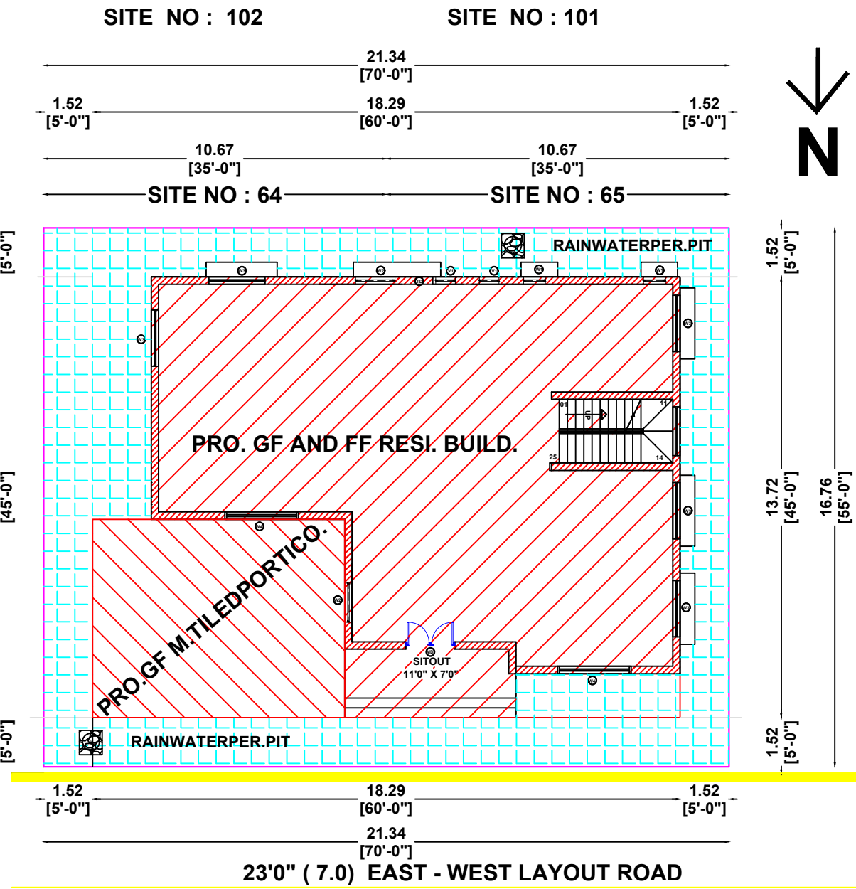
SITE PLAN ( SITE NO : 64 AND 65 )
