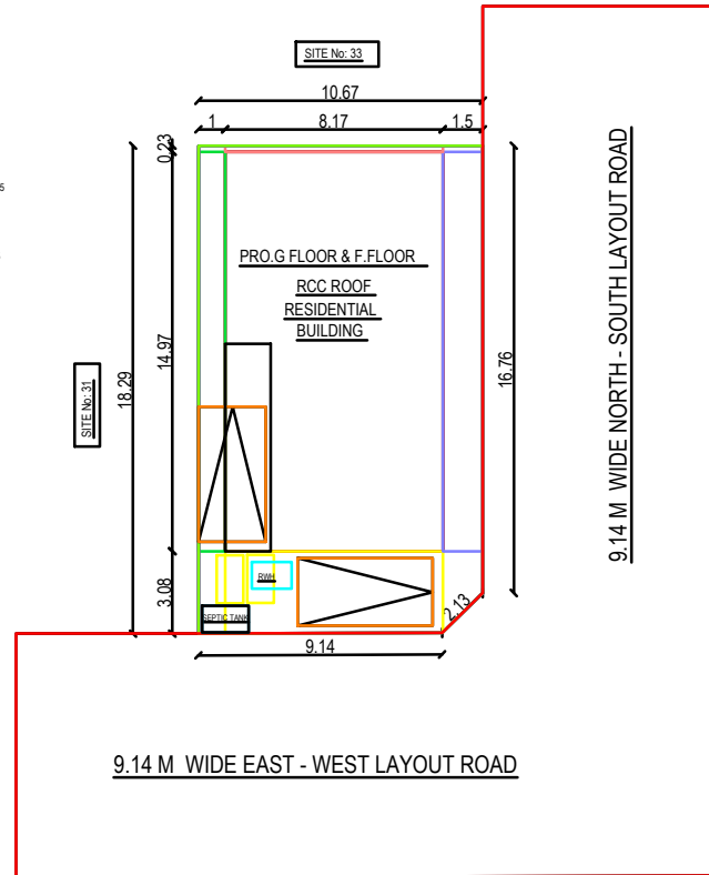
SITE PLAN
