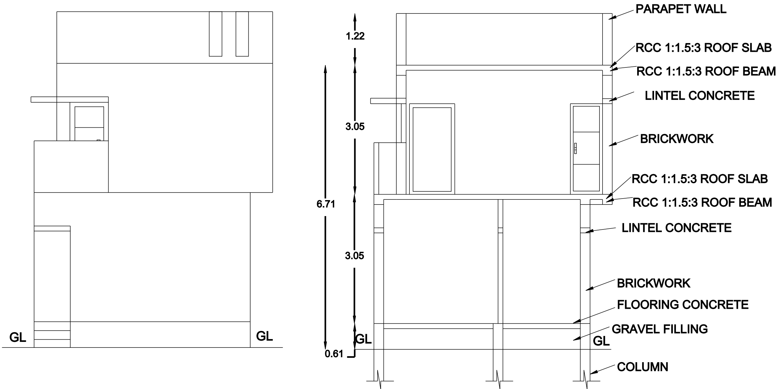
SECTION BB
