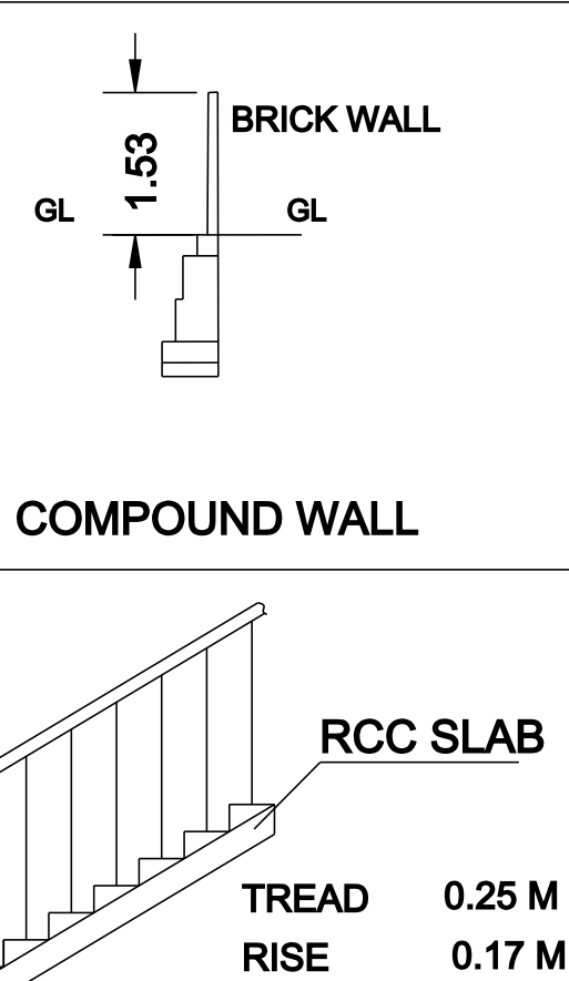
STAIRCASE DETAIL
