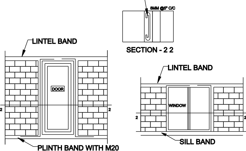
FIGURE 2: REINFORCEMENT AND BENDING DETAILS OF SEISMIC BANDS
