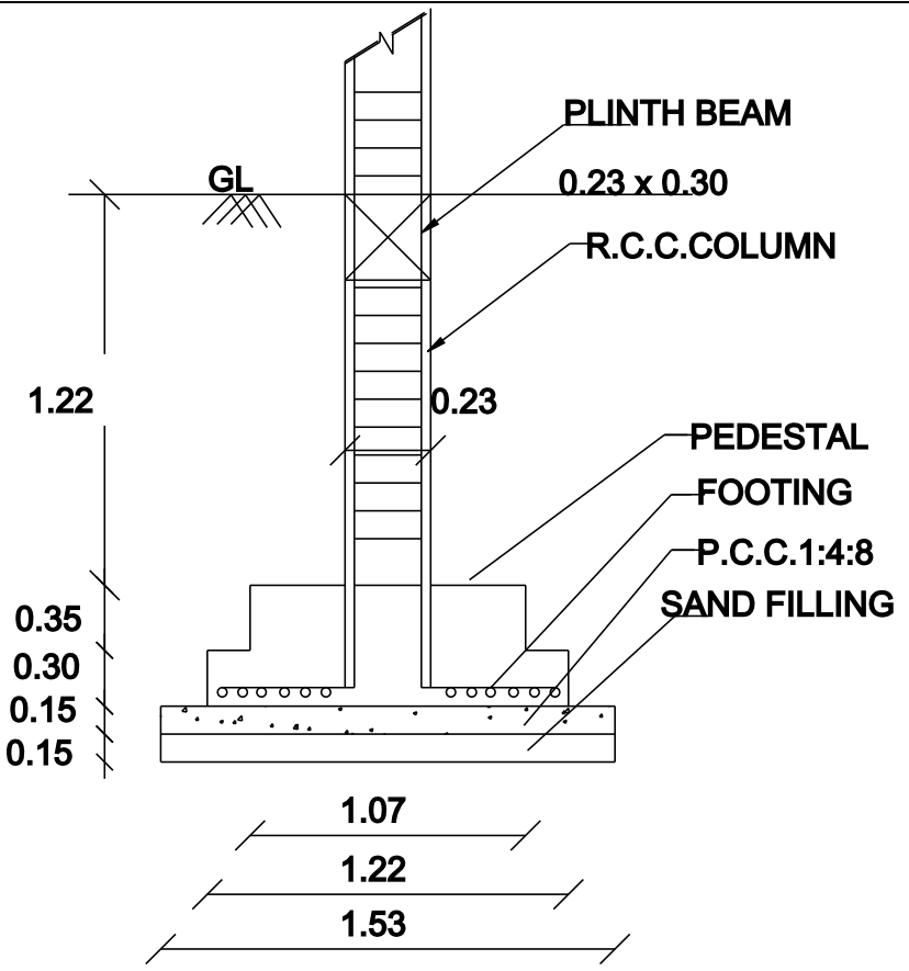
FOUNDATION DETAIL
