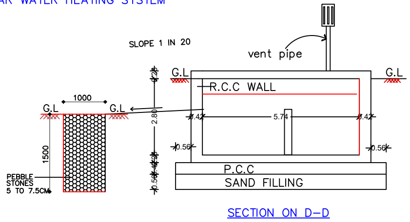
SECTION ON D-D
