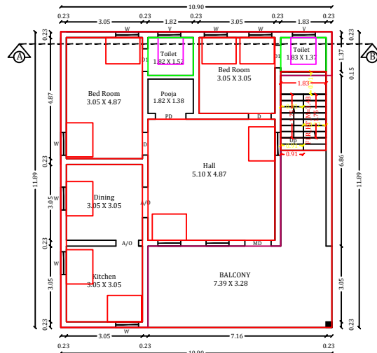
BLOCK 1 PROPOSED FIRST FLOOR PLAN
