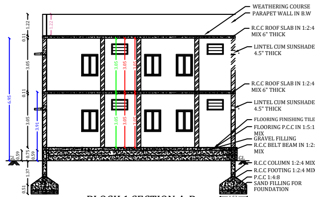
BLOCK 1 SECTION A-B
