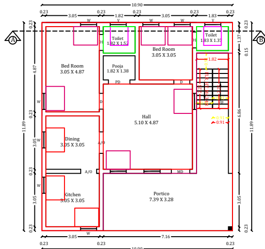
BLOCK-1 EXISTING GROUND FLOOR PLAN
