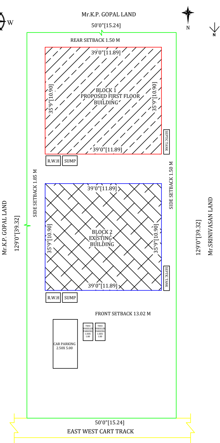
SITE PLAN
