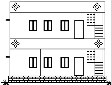
BLOCK 1 ELEVATION
