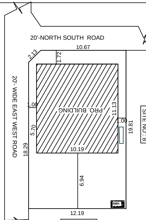
SITE PLAN
