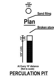
PERCOLATION PIT
