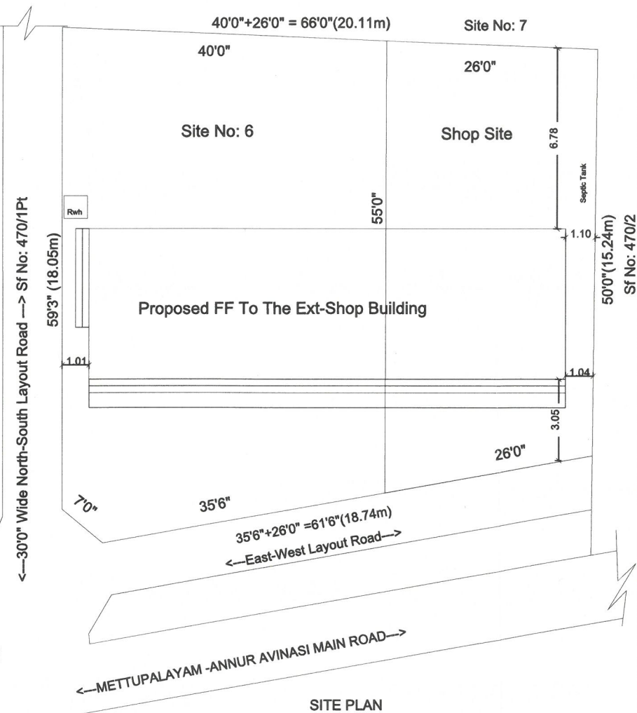
SITE PLAN
