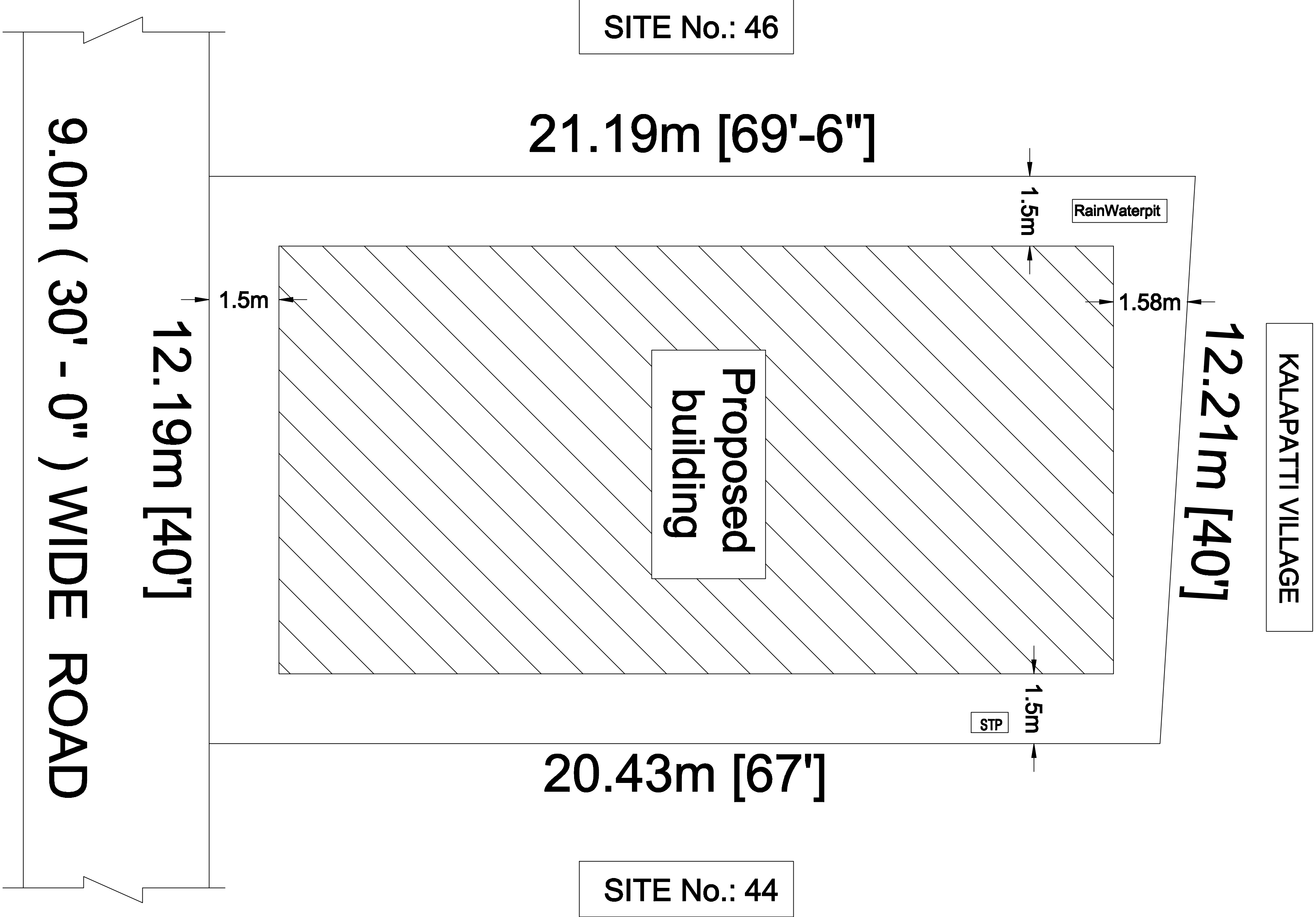
SITE PLAN
