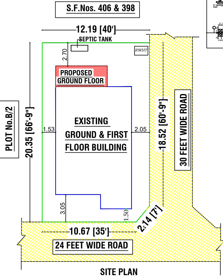
SITE PLAN
