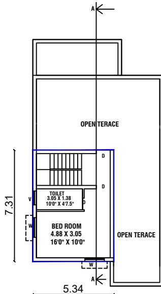
EXISTING FIRST FLOOR
