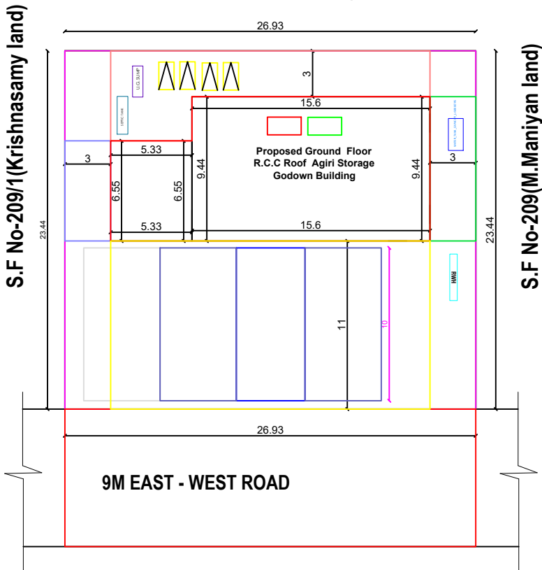
SITE PLAN (SCALE 1" : 8' 0")
