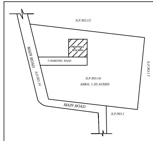
SITE PLAN
