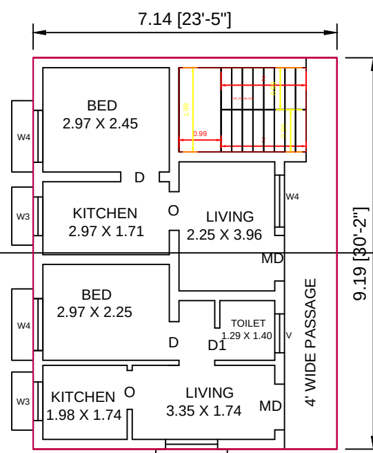
EXI. FIRST FLOOR PLAN
