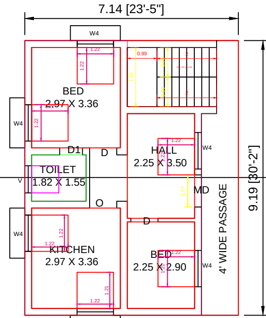
PRO. SECOND FLOOR PLAN
