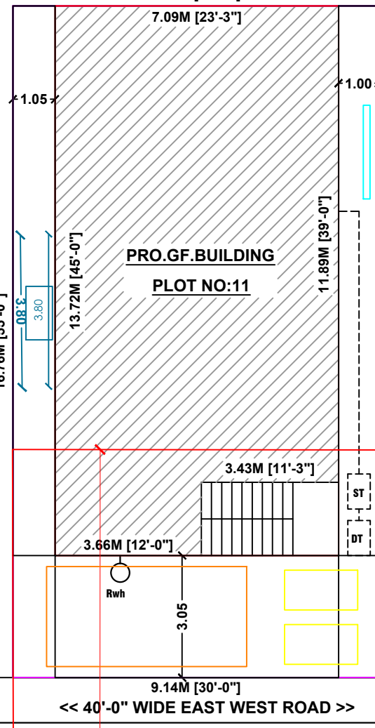
SITE PLAN
