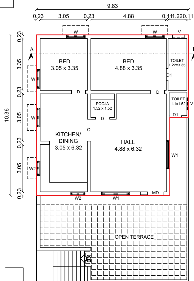
PRO. ADDL. FIRST FLOOR PLAN
