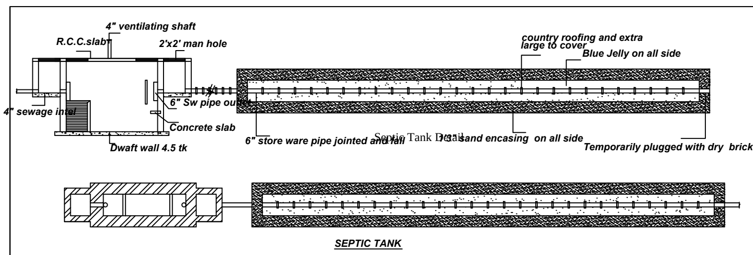
SEPTIC TANK
