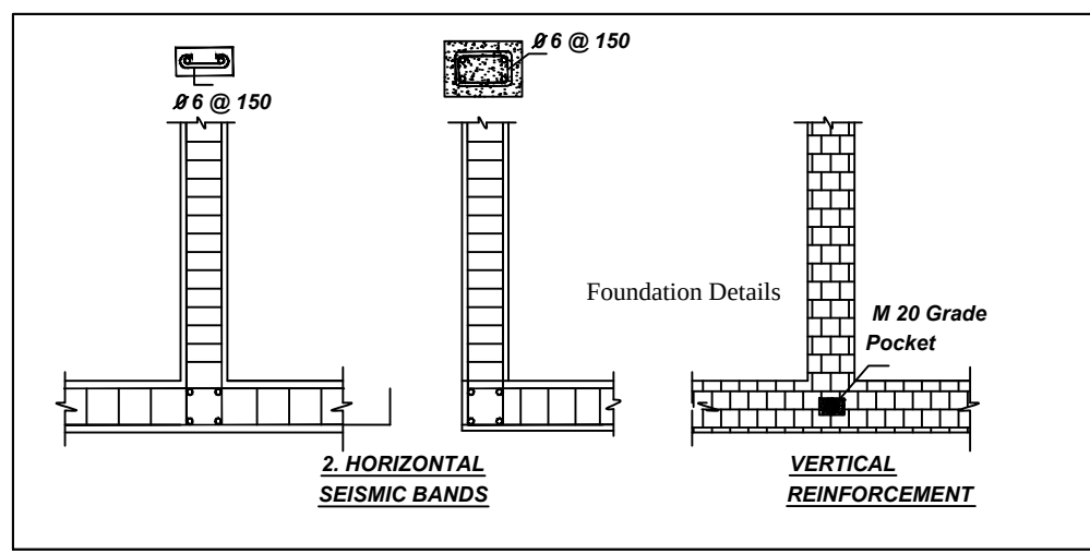
FOUNDATION DETAILS
