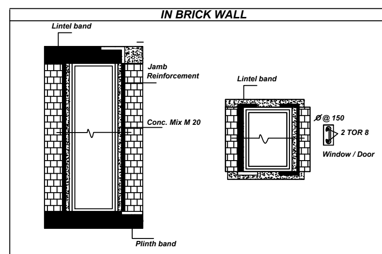
IN BRICK WALL
