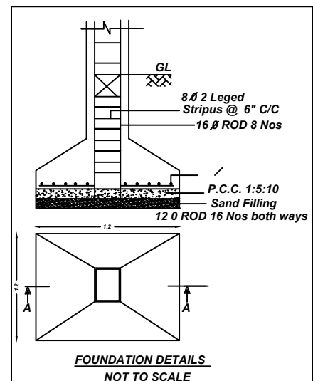
FOUNDATION DETAILS
