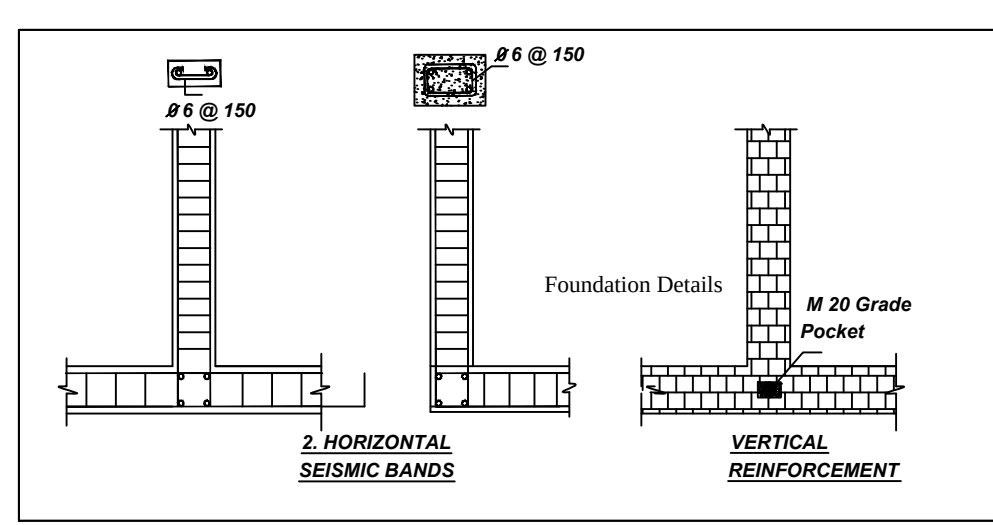
FOUNDATION DETAILS
