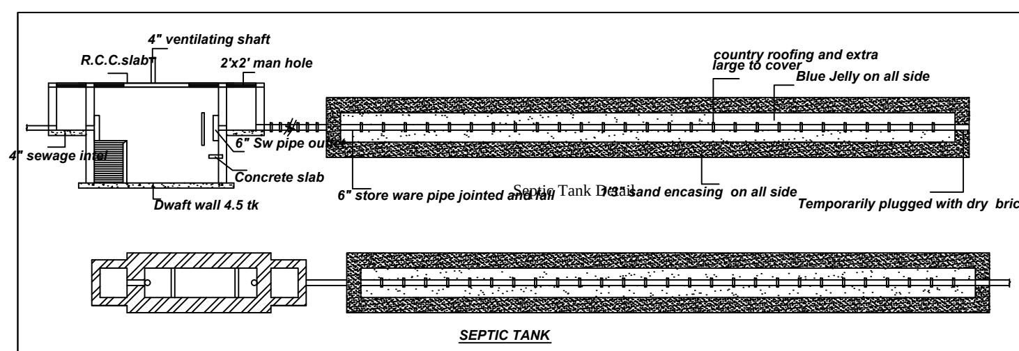
SEPTIC TANK
