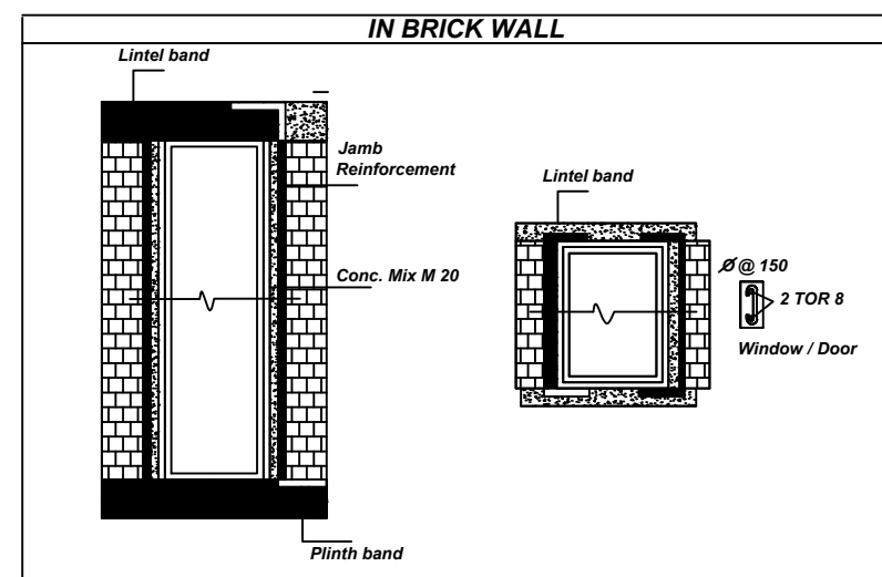
IN BRICK WALL
