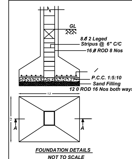
FOUNDATION DETAILS
