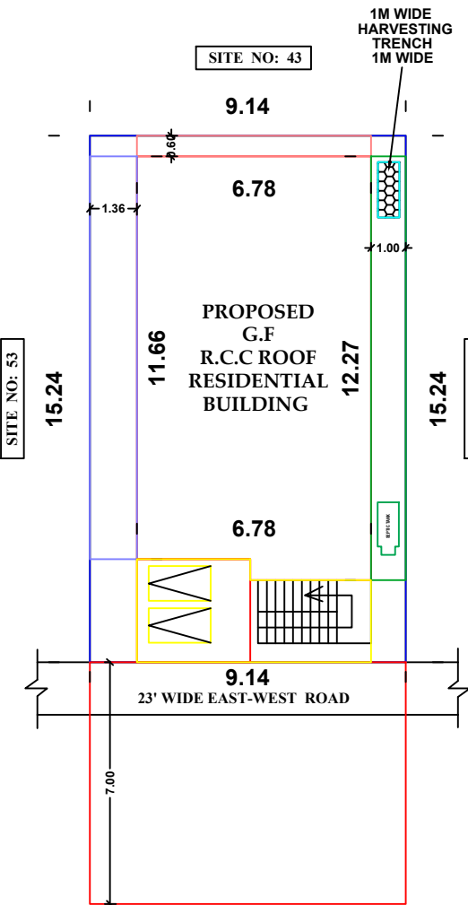
SITE PLAN
