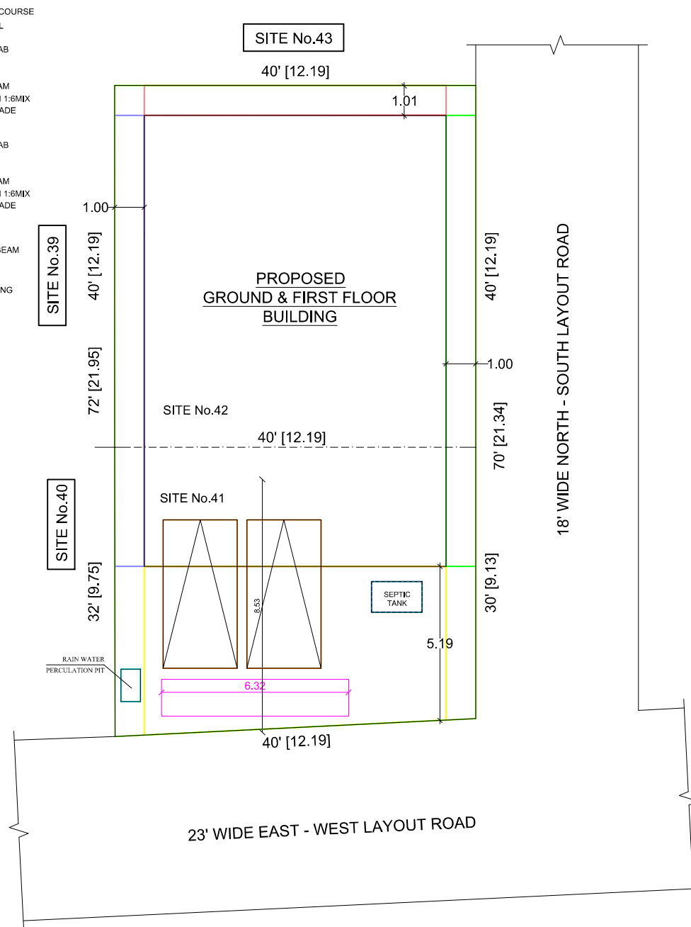
SITE PLAN
