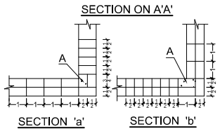
TYPICAL DETAILS OF PROVIDING VERTICAL STEEL BARS IN BRICK MASONRY
