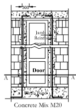
Sectional Elevation OF DOOR
