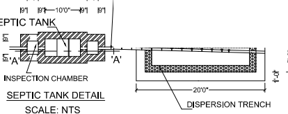
SEPTIC TANK DETAIL SCALE: NTS
