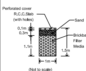
RAIN WATER HARVESTING RECHARGE TRENCH SECTION
