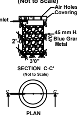
Rain Water Percolation Pit (Not to Scale)
