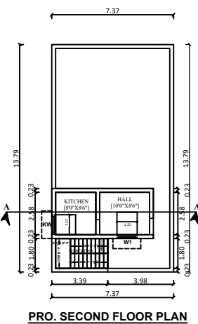
PRO. SECOND FLOOR PLAN
