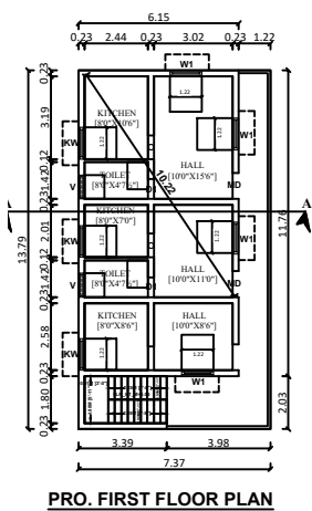
PRO. FIRST FLOOR PLAN
