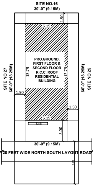
SITE PLAN
