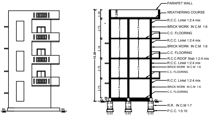
FRONT ELEVATION
