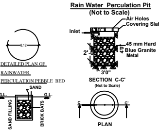
Rain Water Percolation Pit (Not to Scale)
