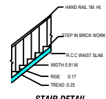
STAIR DETAIL
