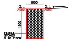
SECTION OF PEBBLE TRENCH SCALE : 1" = 100
