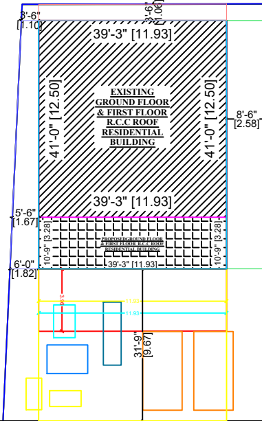
TOPO PLAN
