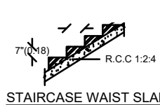
STAIRCASE WAIST SLAB
