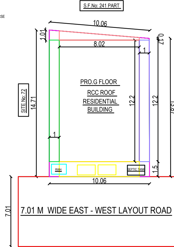
SITE PLAN
