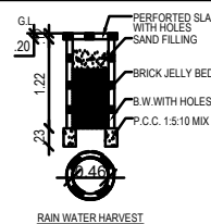
RAIN WATER HARVEST
