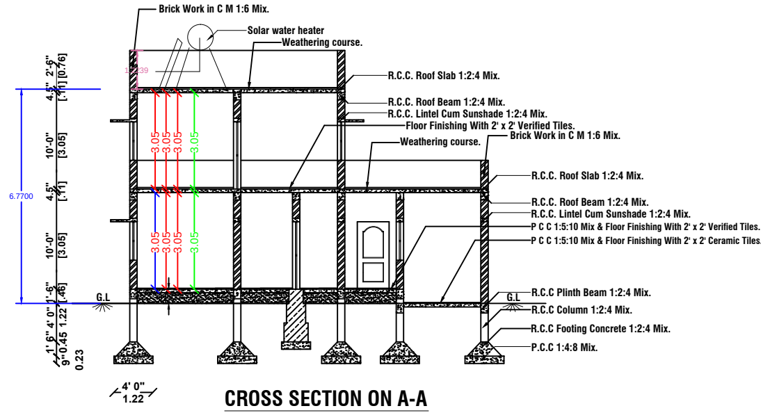
CROSS SECTION ON A-A
