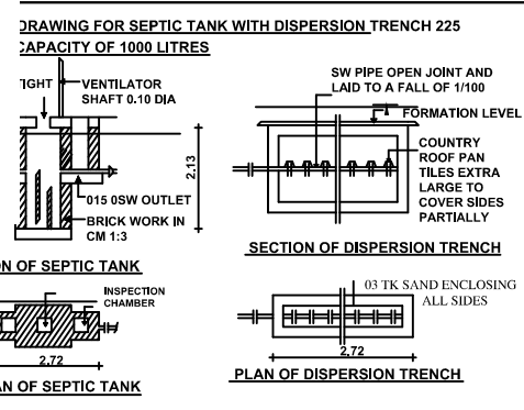
PROPOSED PLAN
