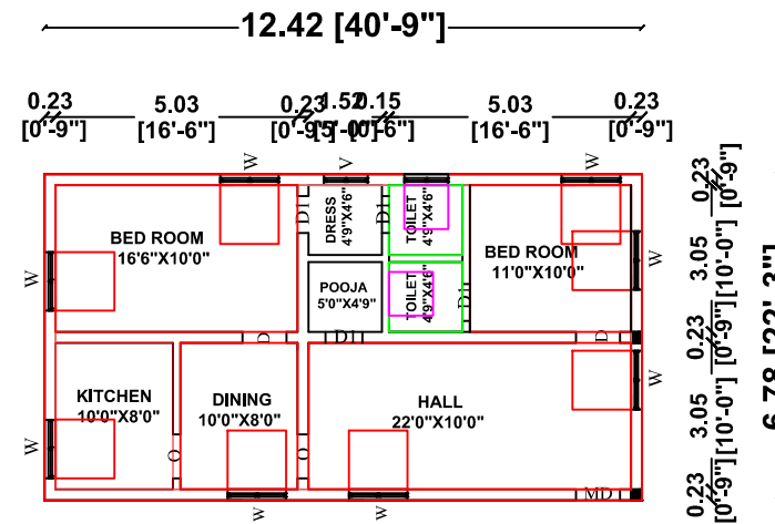
PROPOSED PLAN
