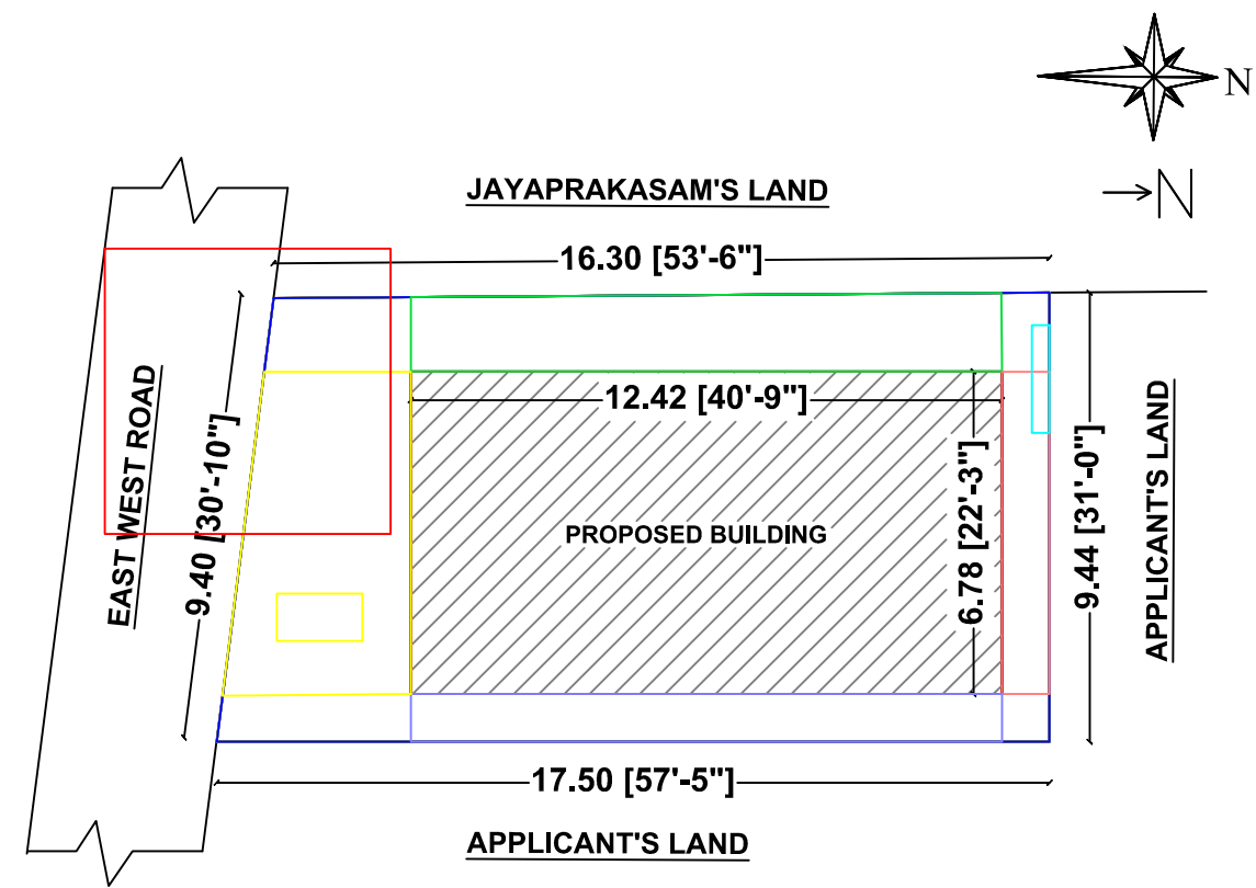
SUPER IMPOSED PLAN
