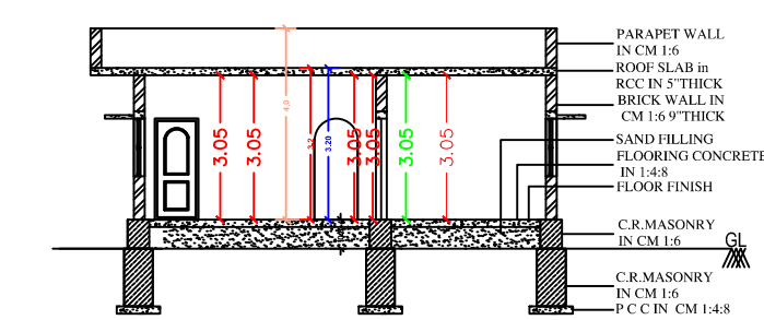
CROSS SECTION
