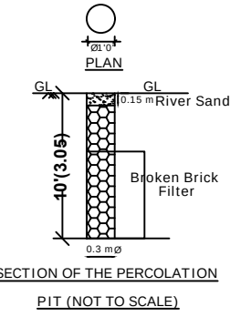
SECTION OF THE PERCOLATION PIT (NOT TO SCALE)
