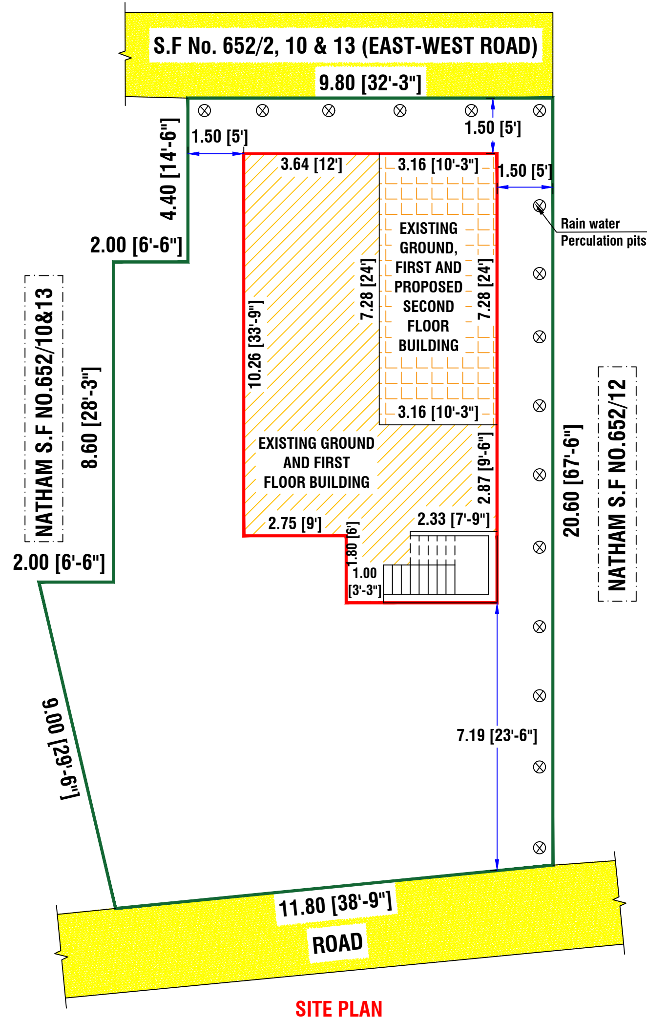
SITE PLAN
