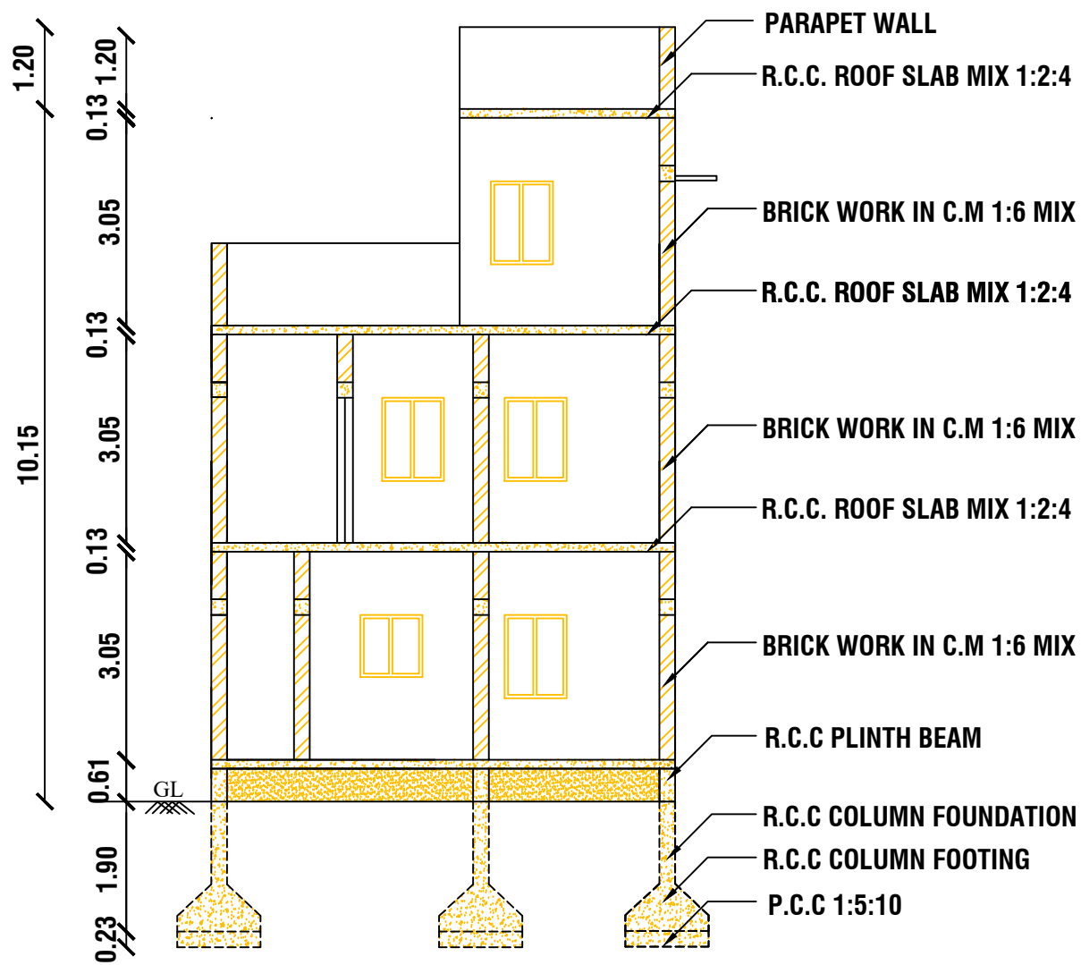
CROSS SECTION AT A-A
