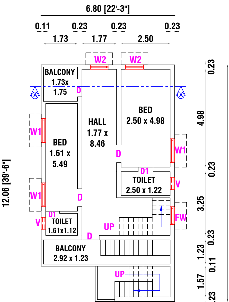
REVISED FIRST FLOOR PLAN
