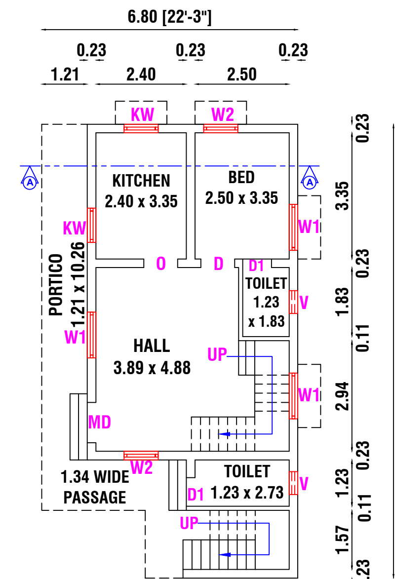
REVISED GROUND FLOOR PLAN
