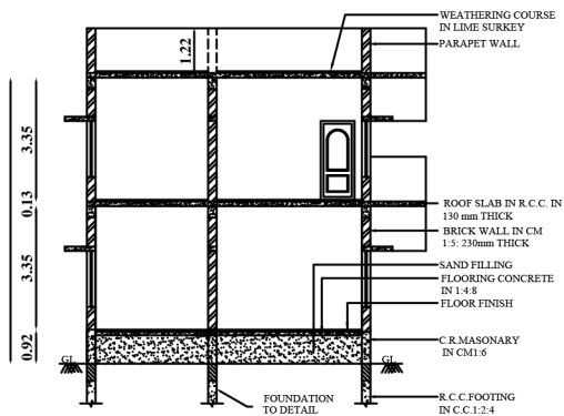
East Side Section On "AB"
