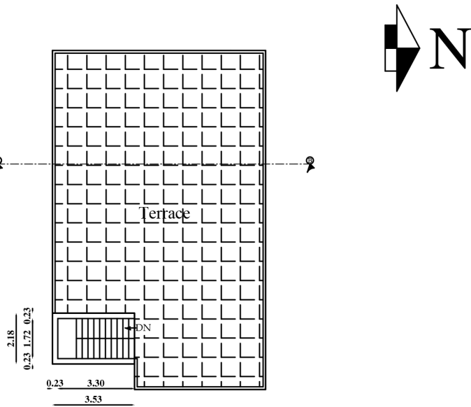
Pro.Head Room Plan
