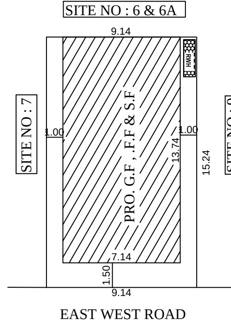
SITE PLAN
