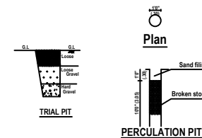
PERCOLATION PIT
