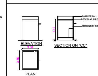
PROPOSED WATCHMAN ROOM
