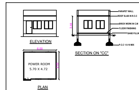
PROPOSED POWER ROOM
