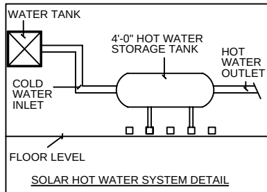
SOLAR HOT WATER SYSTEM DETAIL
