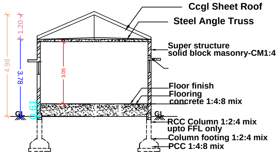
SECTION ELEVATION
