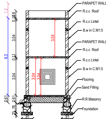
SECTION ON "AB"
