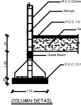
COLUMN DETAIL
