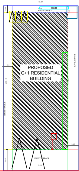
SITE PLAN (SCALE 1:100) 30 FEET ROAD WAY
