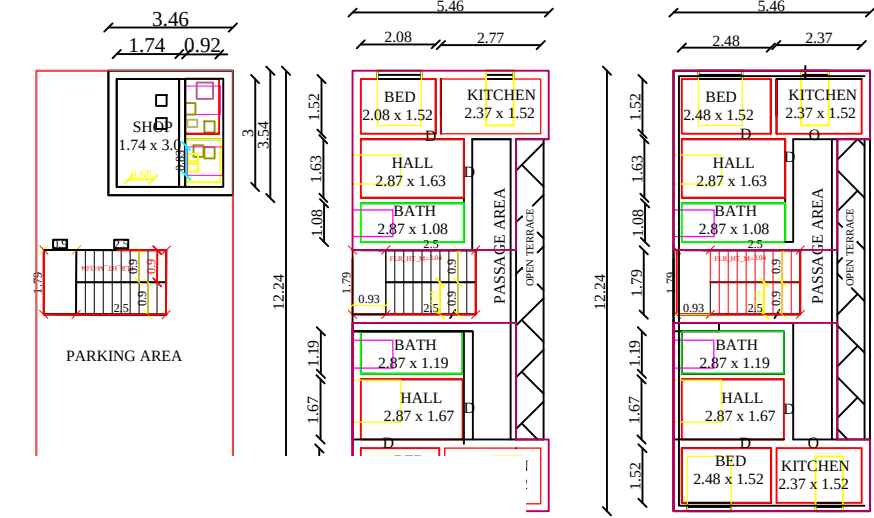
PLAN SECOND FLOOR PLAN
