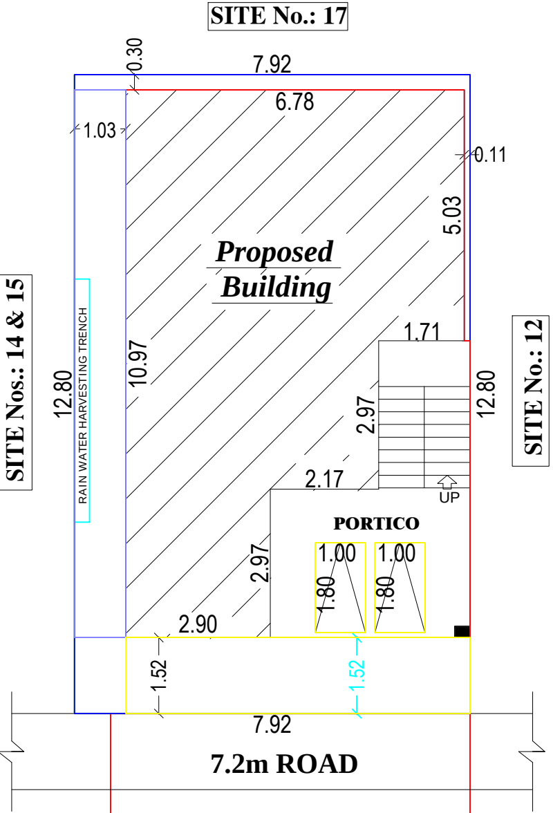
SITE PLAN
