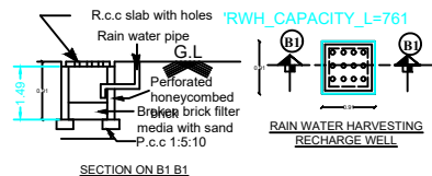
SECTION ON B1 B1
