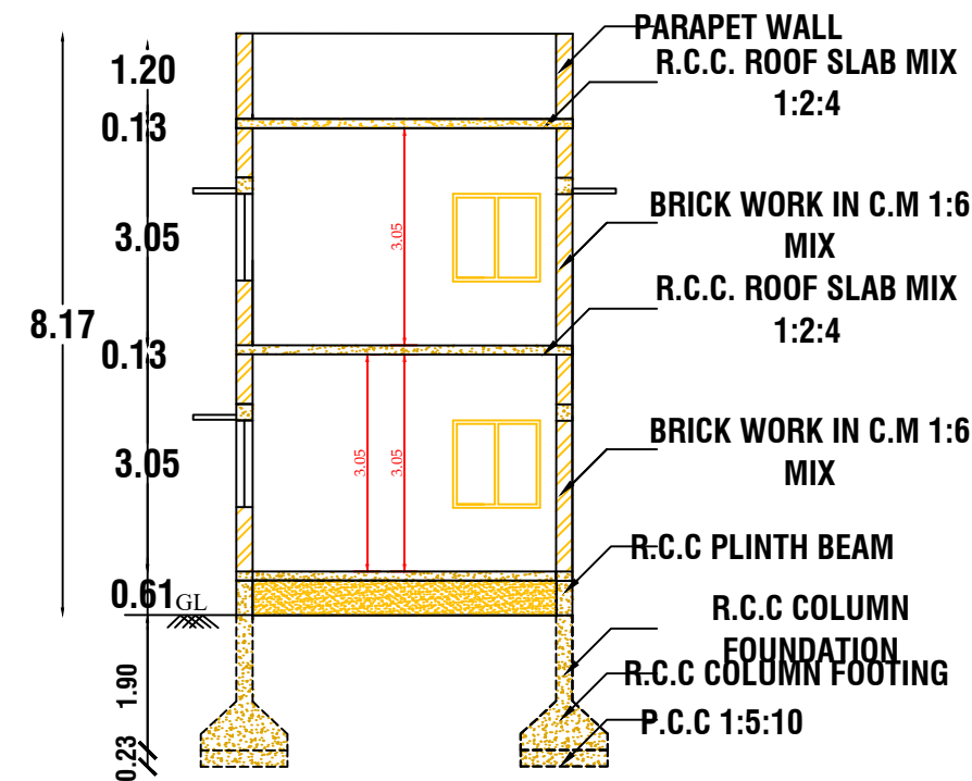
CROSS SECTION AT A-A
