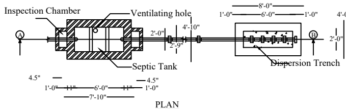
PLAN
