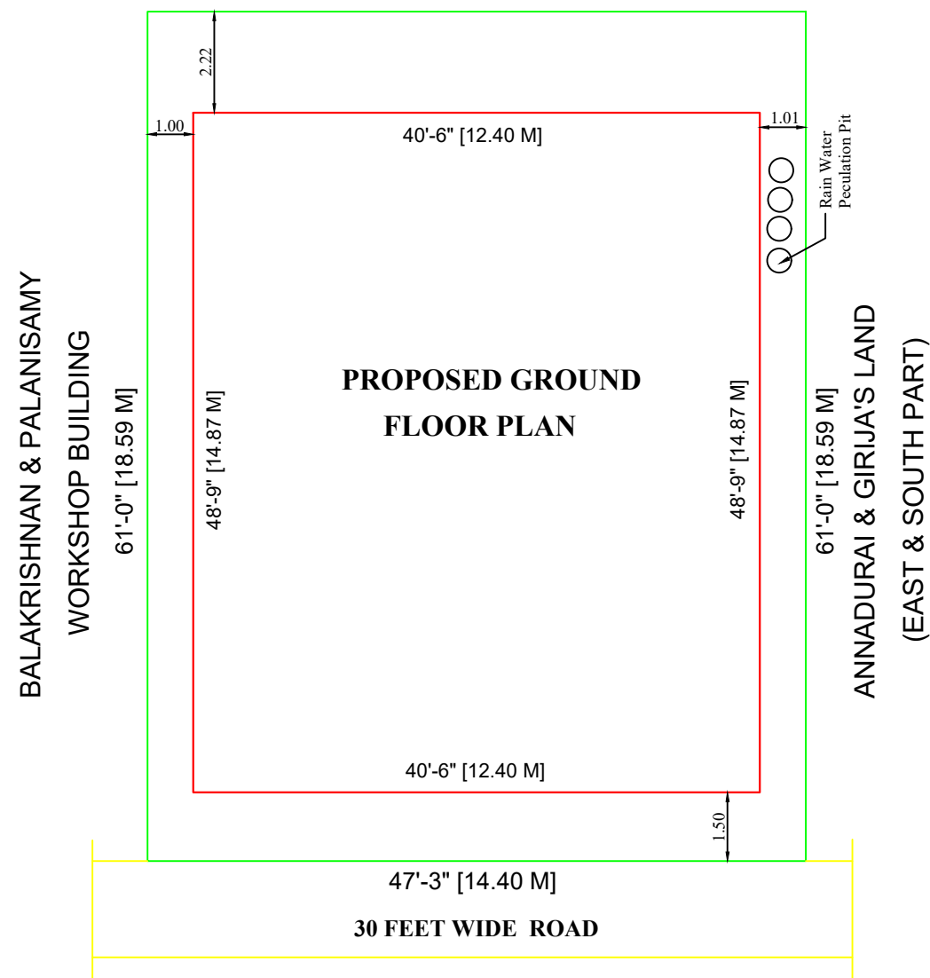
SITE PLAN
