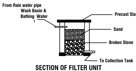
SECTION OF FILTER UNIT
