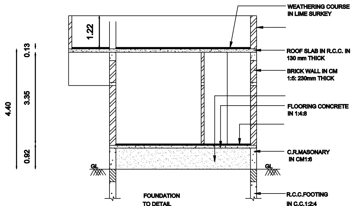
Eastern Side Section On "AB"
