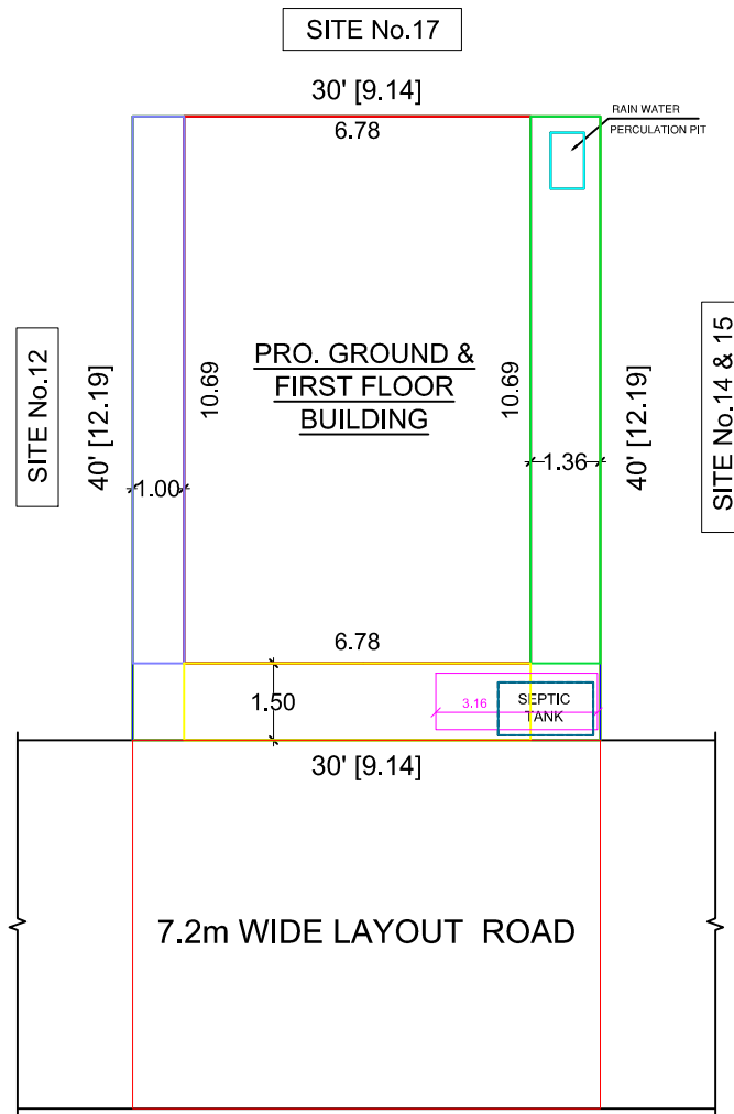
SITE PLAN
