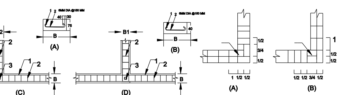
FIGURE 2: REINFORCEMENT AND BENDING DETAILS OF SEISMIC BANDS
