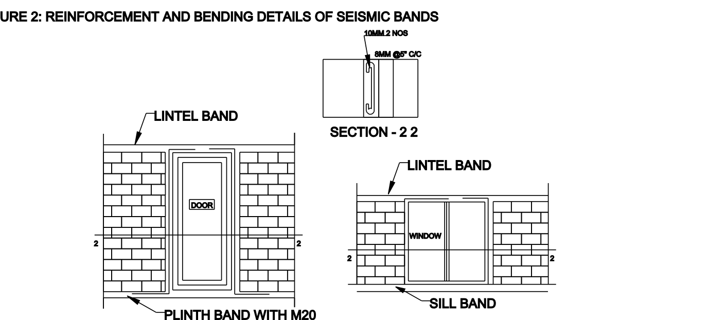
FIGURE 2: REINFORCEMENT AND BENDING DETAILS OF SEISMIC BANDS
