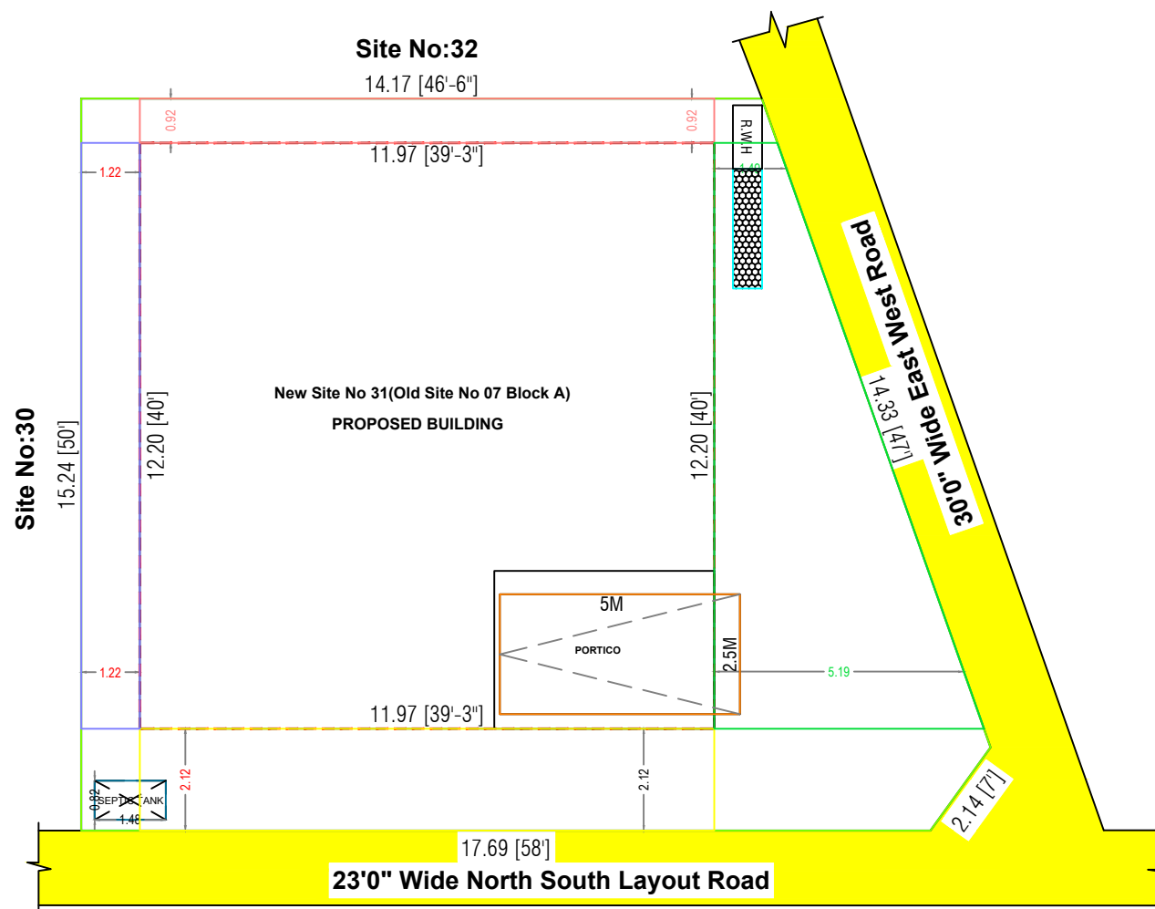
SITE PLAN
